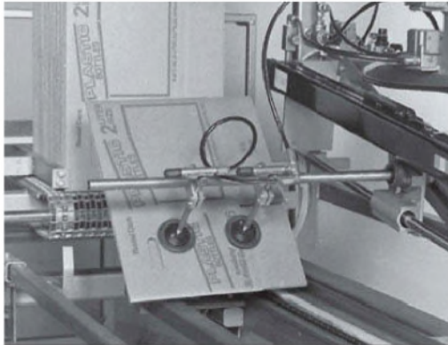
JD-100M – carton erecting application
