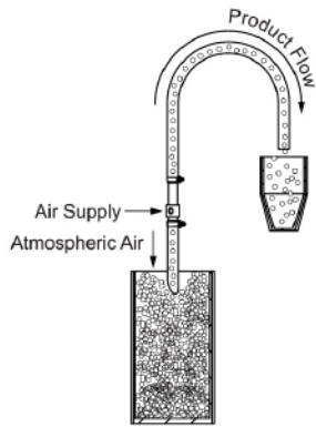
Basic Hopper
