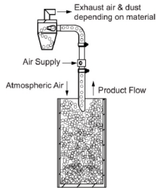
Hopper Inlet
