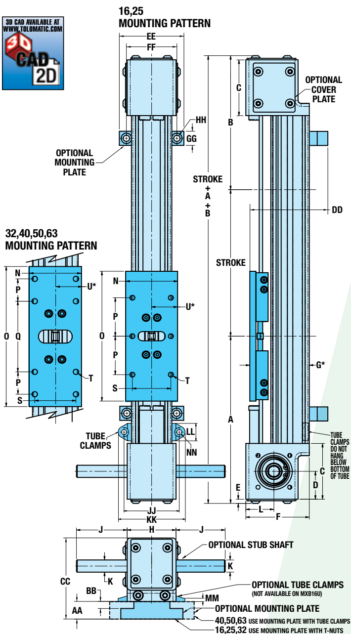
OPTIONAL MOUNTING PLATES
