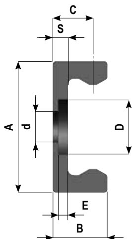
MR..L Counterbored holes
