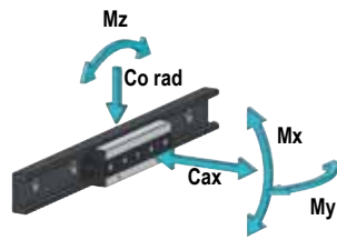
5 Rollers slider for R. series
