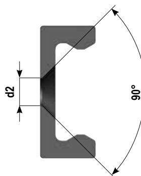
MR..S Countersunk holes
