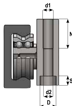
RVT Guiding slider dimensions
