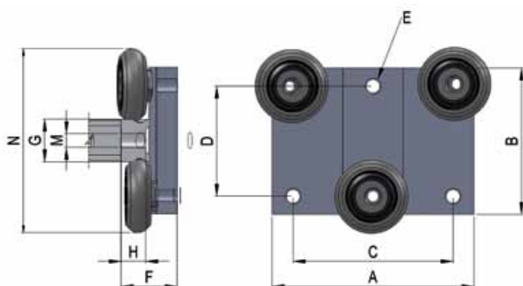
Slider series RBS
