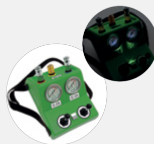
DOUBLE DEADMAN CONTROLLER 10 bar – LED LIGHTS, PLASTIC BOX 291286
