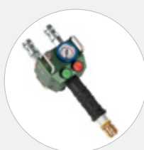
HAND-HELD DOUBLE DEADMAN CONTROLLER 10 bar 291257
