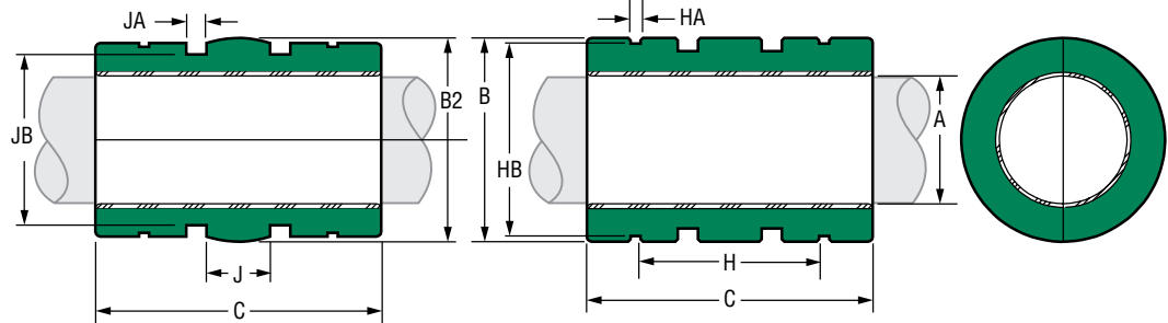
*Self Aligning O.D. (FJA-XX)
