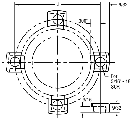
Dimension for calculating bolt circle: J = C + .600
